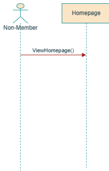
Figure 25: Sequence Diagram for View Homepage
