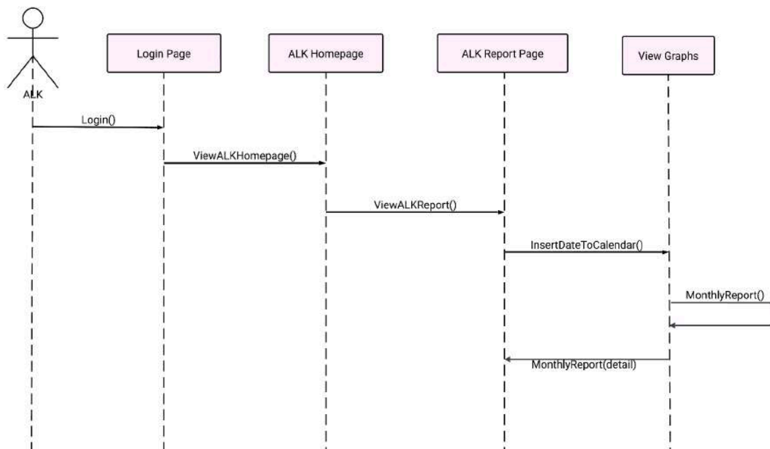
Figure 22: Sequence Diagram for View Monthly Report
