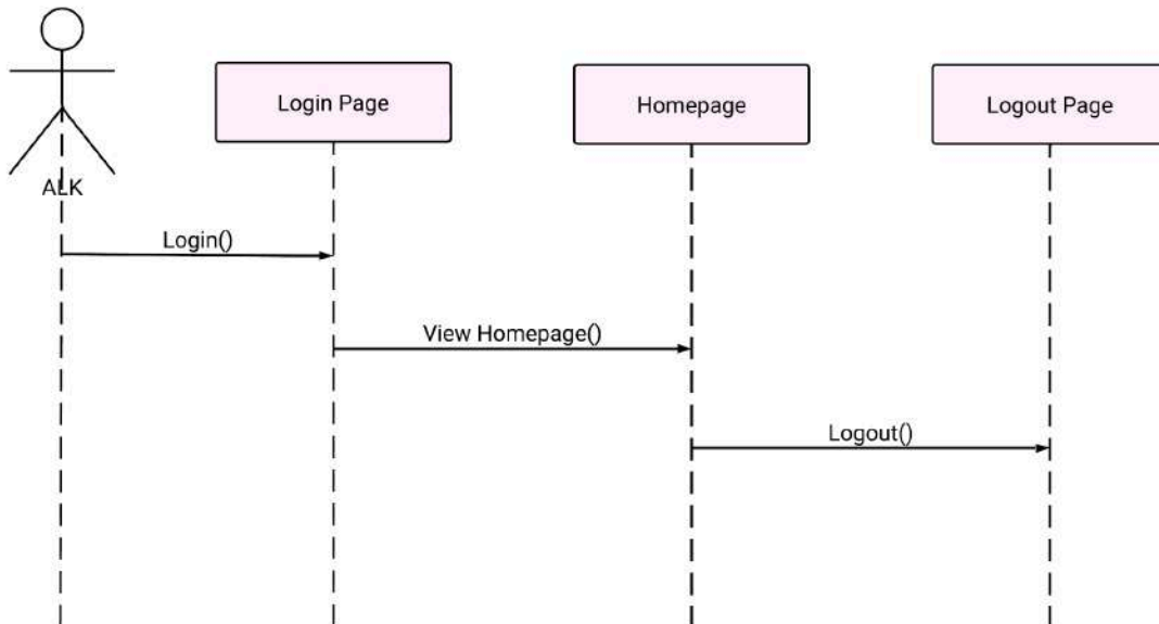
Figure 28: Sequence Diagram for Log Out
